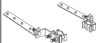
UNIVERSAL EAVE BRACKET EB2525G
