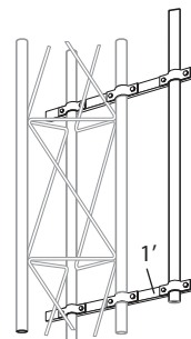
DBS ANTENNA MOUNT KY2068A16 - 1.66" O.D. KY2068A15 - 1.50" O.D. KY2068A2 - 2.38" O.D.
