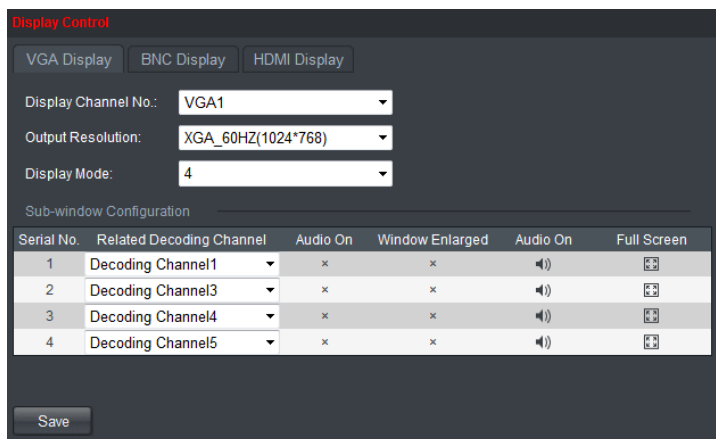
Figure 4.3 Display Configure
