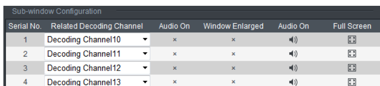
Figure 4.5 Sub-window Information
