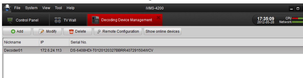
Figure 5.16 Decoder List
