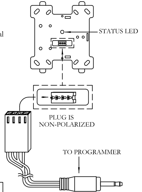
FIGURE 1. EXPLODED VIEW OF ADDRESS PROGRAMMING-PLUG AND CONNECTOR
