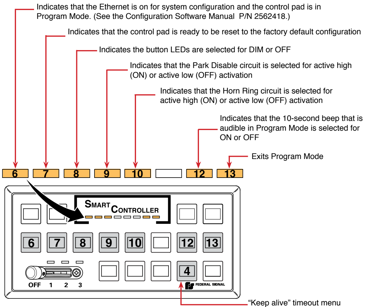
Figure 6.1 LEDs and buttons associated with Program Mode settings
