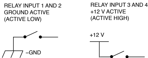
Figure 3.8 Switch operation for Inputs 1 to 4
