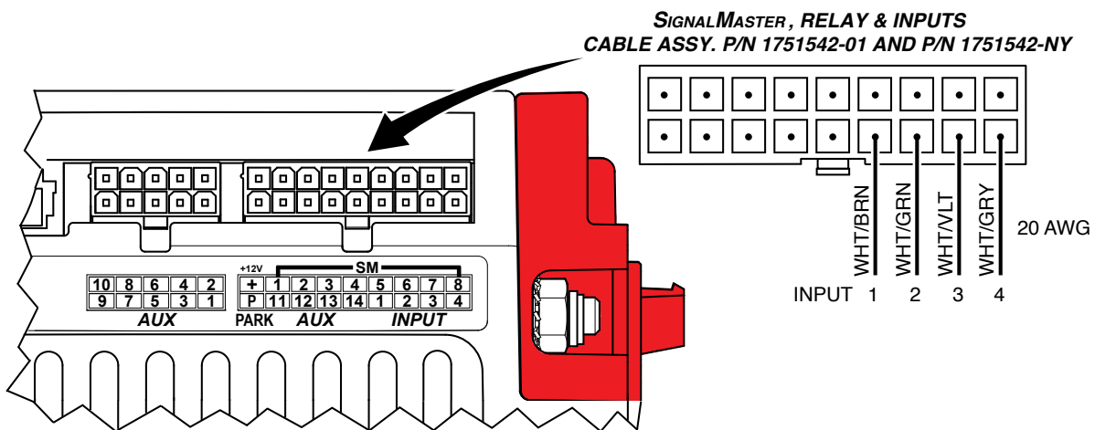
Figure 3.9 Connections for discrete-wire SignalMaster
