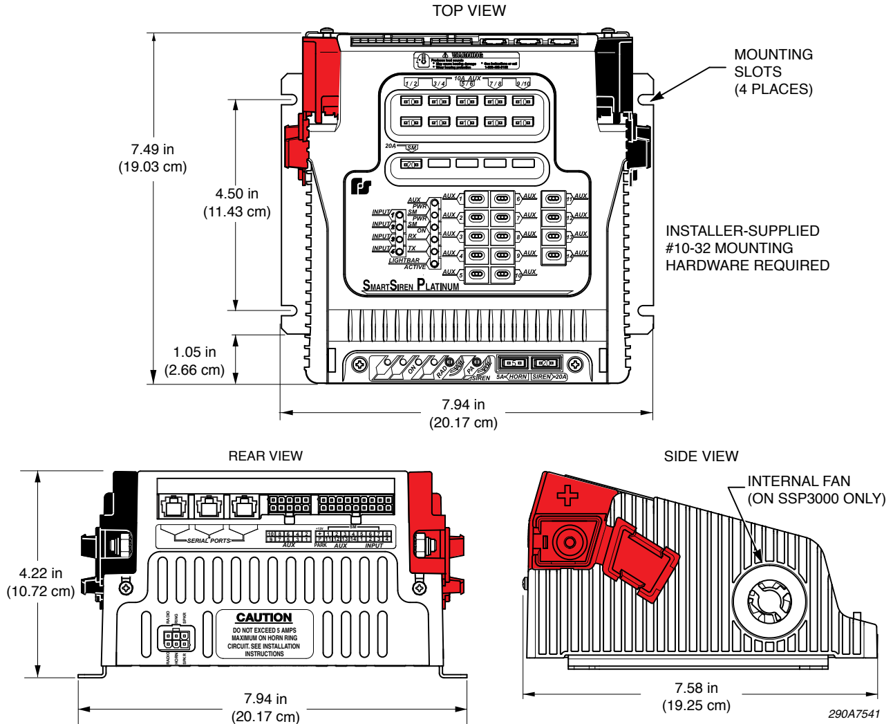
Figure 3.2 Dimensions of the siren amplifier/relay module
