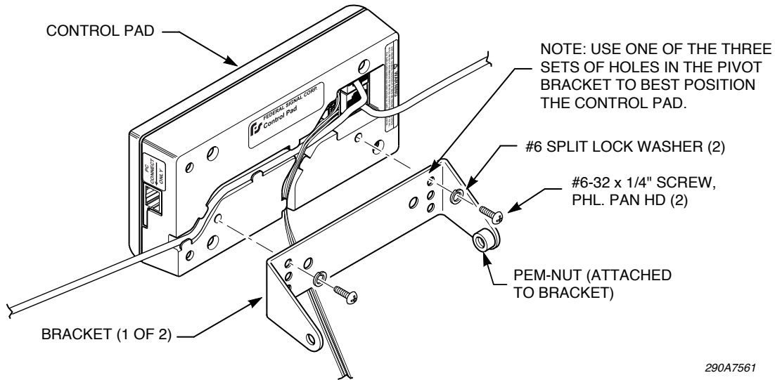
Figure 5.2 Bracket attached to back of control head
