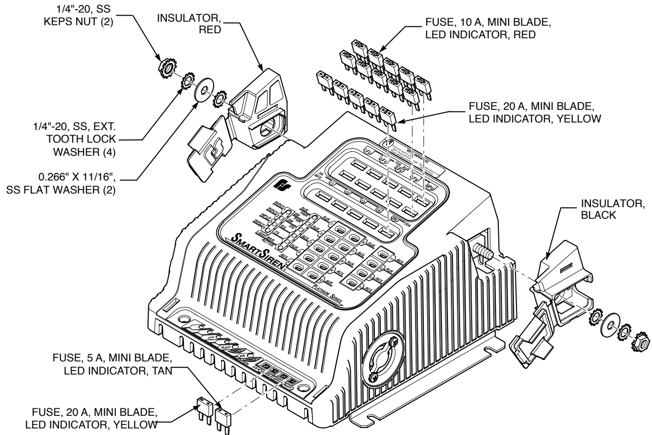
Figure 10.4 External parts assembly (SSP3000B shown)
