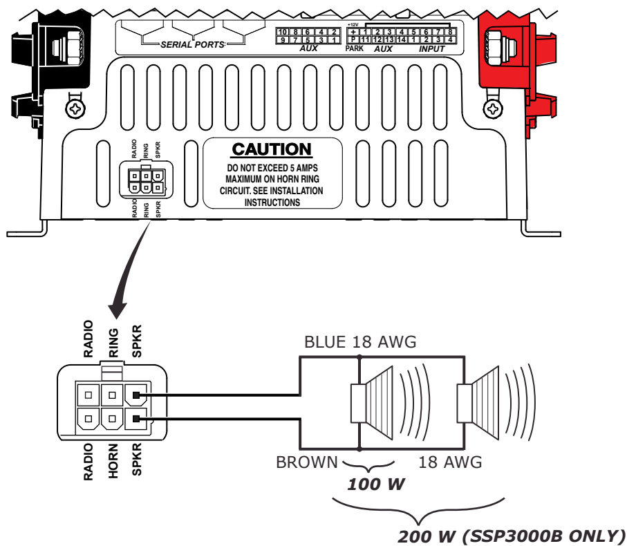
Figure 3.11 Connections for two speakers
