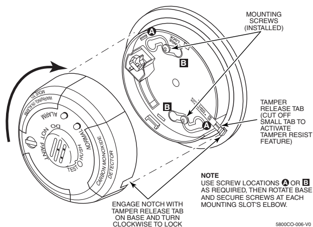
Figure 2. Mounting the Detector
