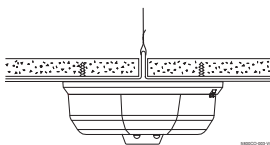
Figure 3. Mount Detector Across Ceiling Panel Support
