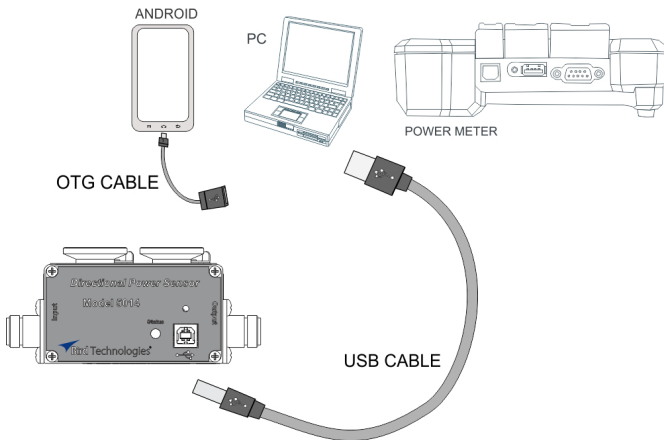
Figure 3 5014 Cable Connections
