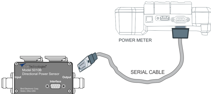
Figure 2 5010 Cable Connection
