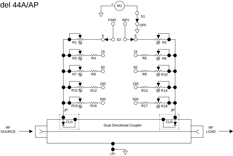
Figure 3-1: Model 44A/AP RF Wattmeter Schematic
