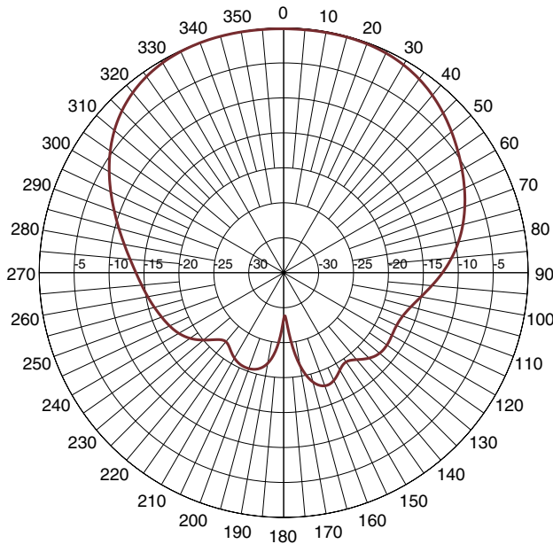
PORT 2-2450 MHz-E-plane
