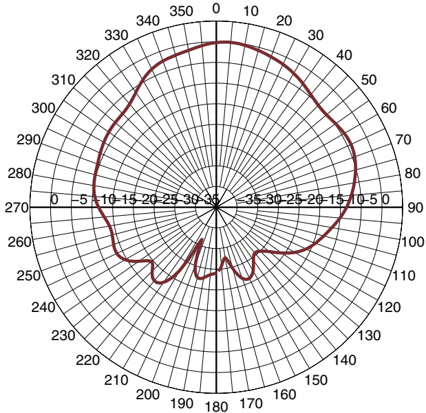
5 GHz-E-plane
