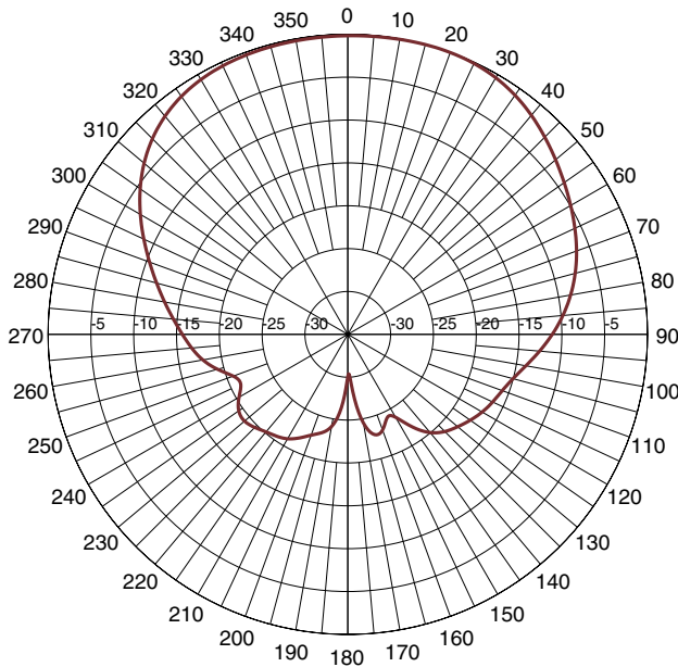
PORT 3-2450 MHz-E-plane
