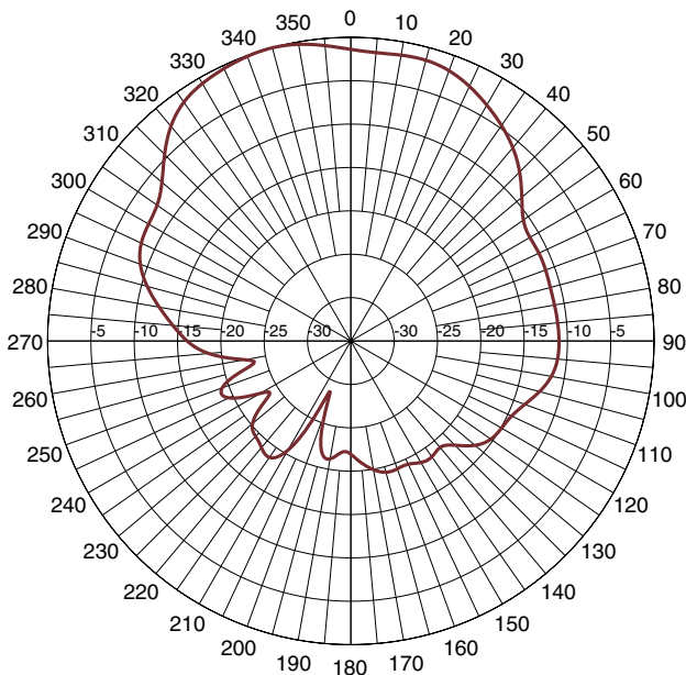
PORT3-5000 MHz-E-plane
