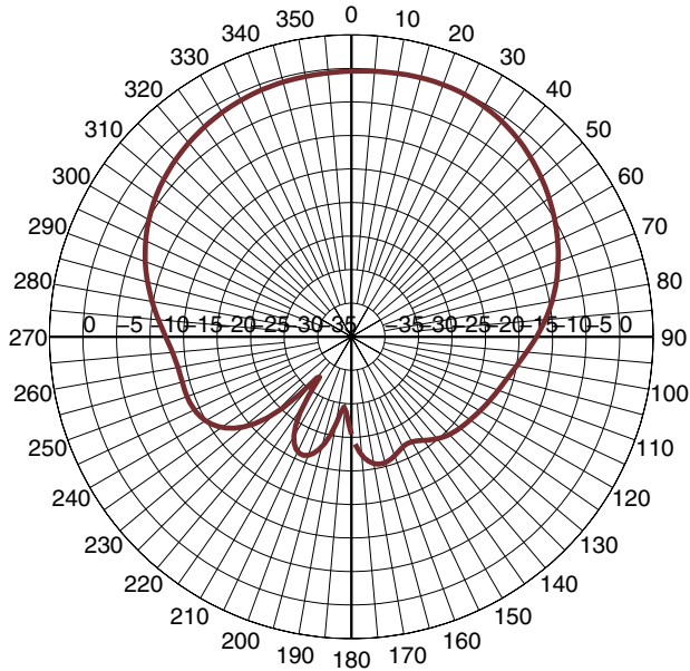
2.5 GHz-E-plane
