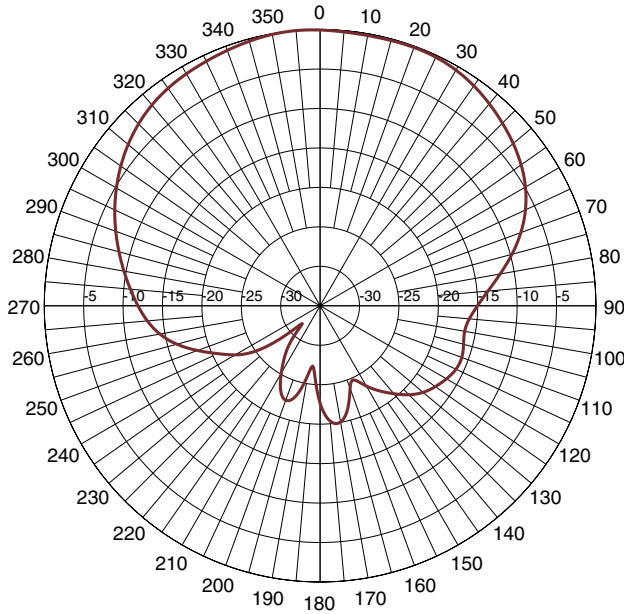
PORT 4-2450 MHz-E-plane
