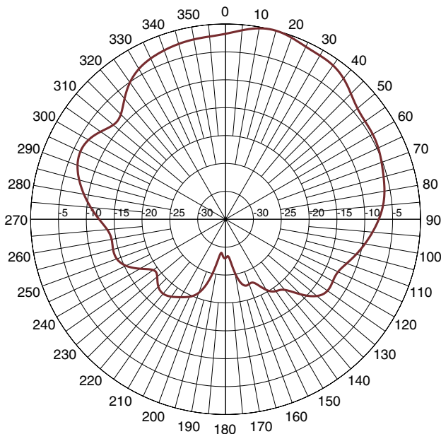
PORT 2-5000 MHz-E-plane
