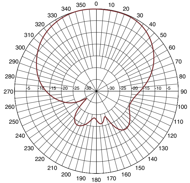
PORT 4-2450 MHz-H-plane
