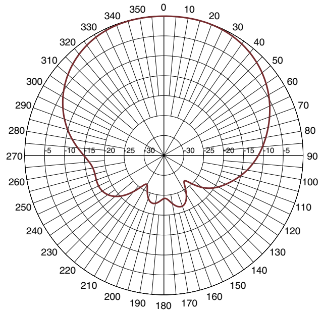
PORT 1-2450 MHz-H-plane
