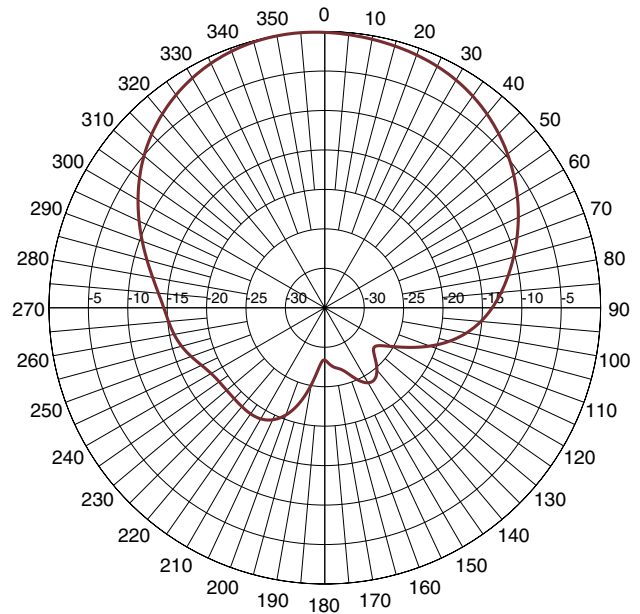
PORT 2-2450 MHz-H-plane
