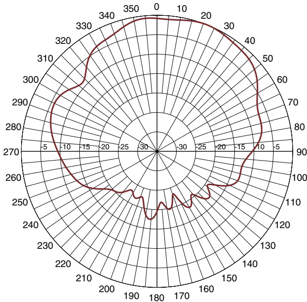
PORT 4-5000 MHz-E-plane
