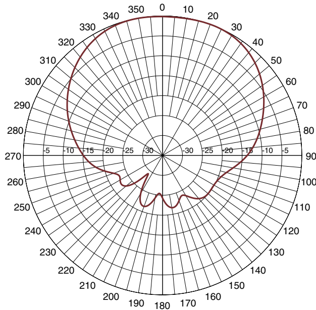
PORT 1-2450 MHz-E-plane
