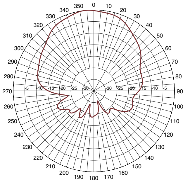
PORT 1-5000 MHz-E-plane
