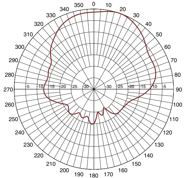
PORT4-5000 MHz-H-plane
