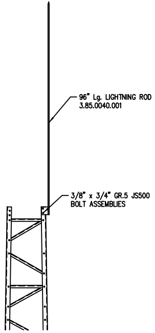
LIGHTNING ROD KIT P/N 4.90.0100.000
