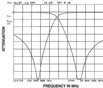
636-6A RESPONSE CURVES (Typical) 4.5 MHz SPACING (136-174 MHz)
