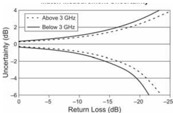
Figure 6 Match Measurement Uncertainty
