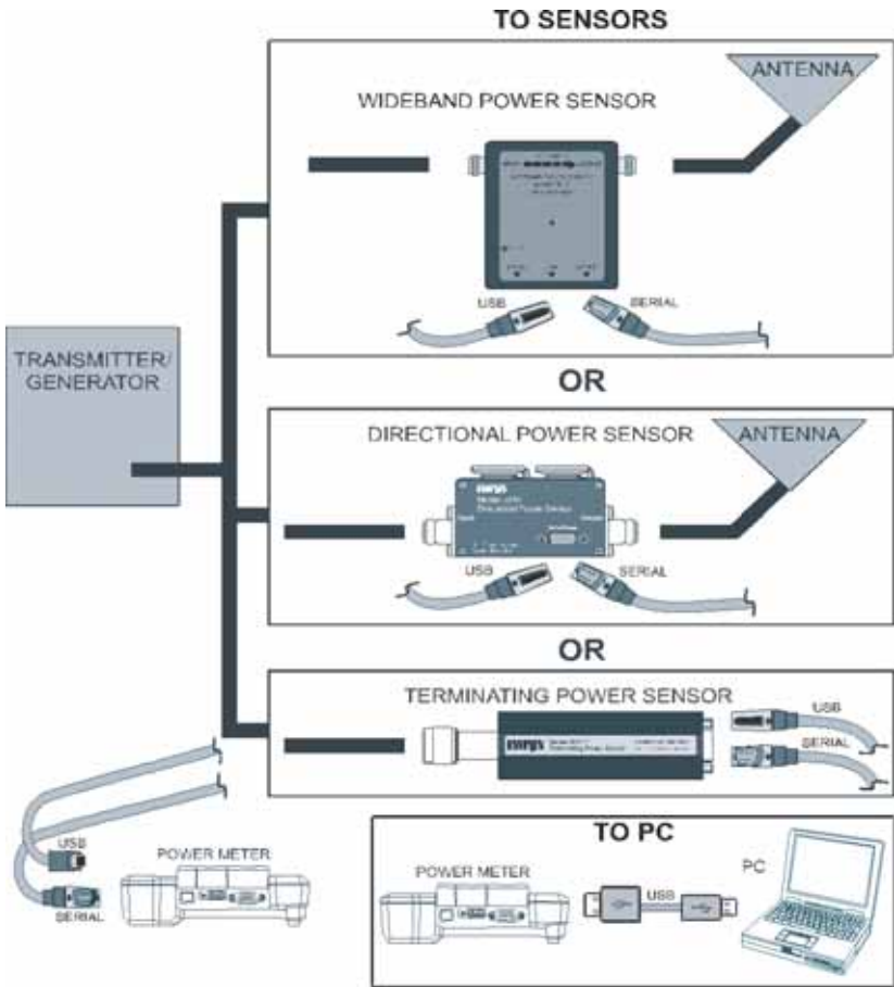
Figure 3 DPM Connections
