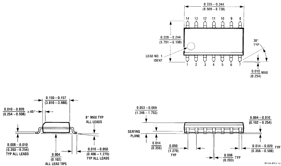
14-Pin Small Outline Package Order Number LMC6494AEM or LMC6494BEM NS Package Number M14A
