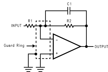
Inverting Amplifier
