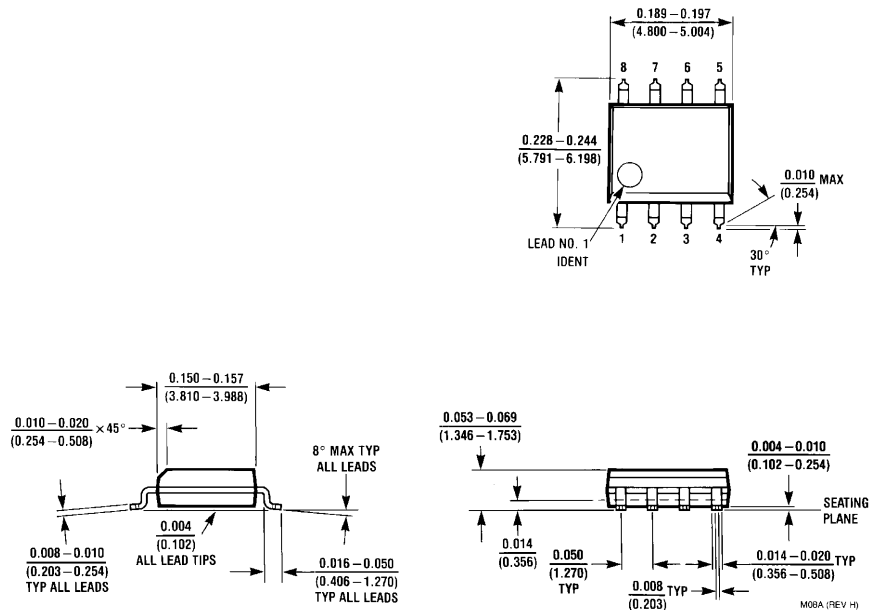
8-Pin Small Outline Package Order Number LMC6492AEM or LMC6492BEM NS Package Number M08A
