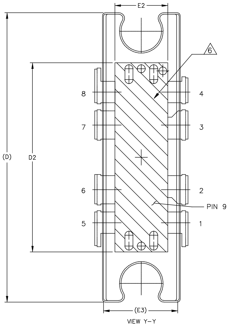
VIEW Y-Y
