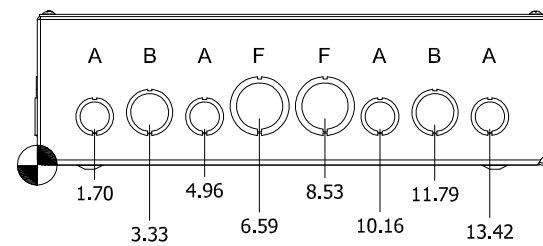
BOTTOM VIEW
