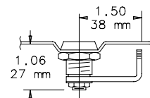
Cylinder Lock Kit AL12AR (optional)
