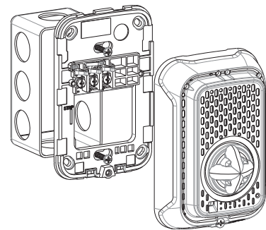
Figure 9 Mounting a Compact Wall Device (Single-gang box)
