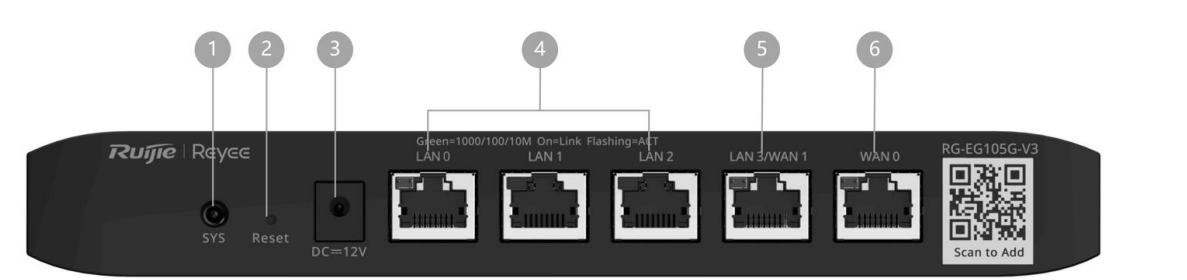
Figure 1-2 Front Panel of RG-EG105G-V3
