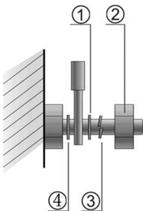
Figure 6-8 Cable Fastening
