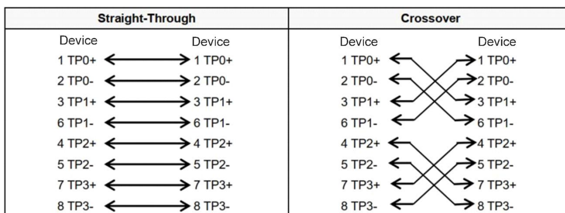
Figure 6-1 1000BASE-T Connection
