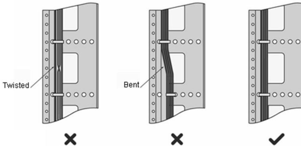
Figure 6-4 Binding Cables (1)
