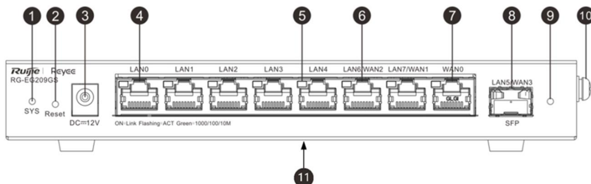
Figure 1-2 Front Panel of an RG-EG209GS Router
