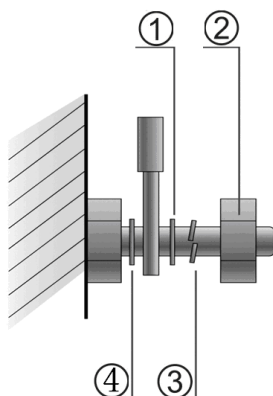
Figure 6-7 Cable Fastening
