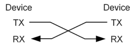
Figure 6-3 Fiber-Optic Cable Connection
