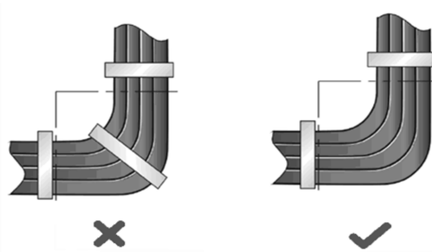
Figure 6-6 Binding Cables (3)
