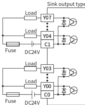
Figure 12 Transistor output equivalent circuit
