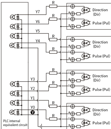
Figure 13 Pulse output wiring diagram
