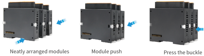
Figure 7 Snap-in installation
