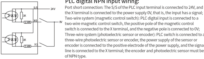
Figure 9 Input wiring diagram
