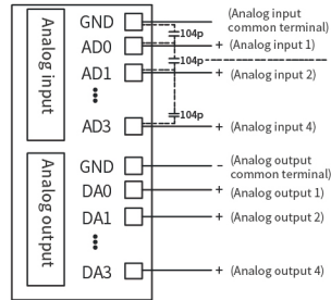
Figure 14 PLC analog wiring
