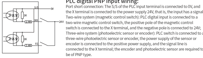
Figure 10 Input wiring diagram
