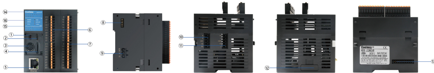
Figure 1 Product structure
