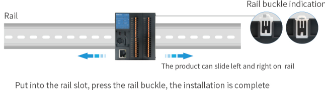
Figure 8 Rail installation
