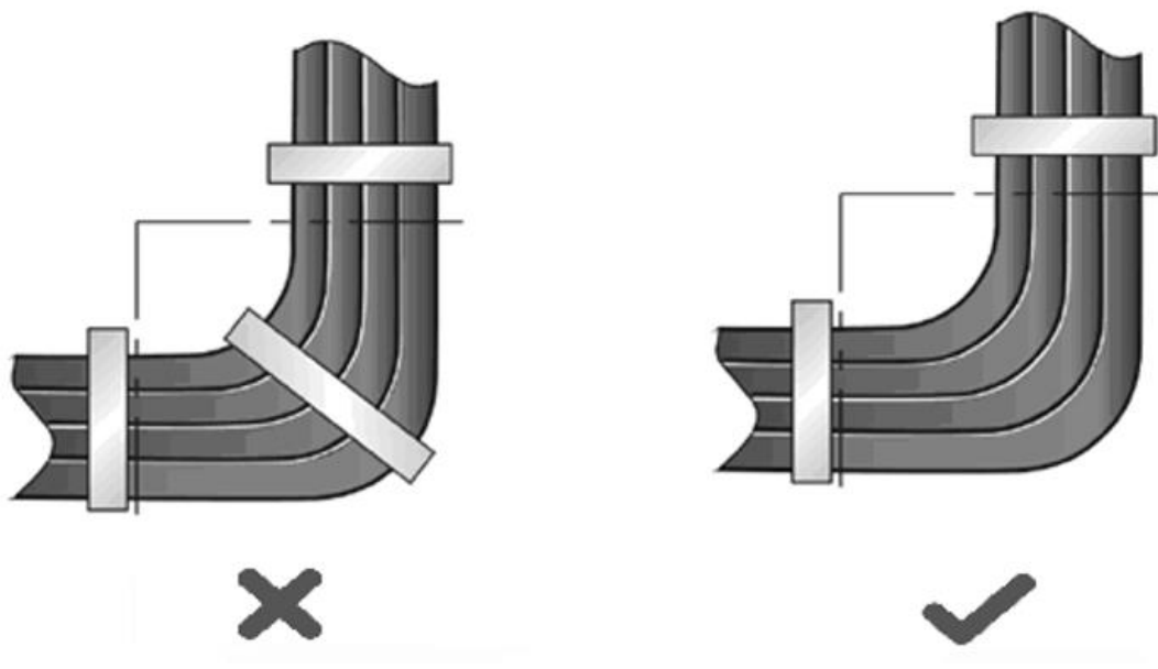
Figure 6-8 Binding Cables (3)
