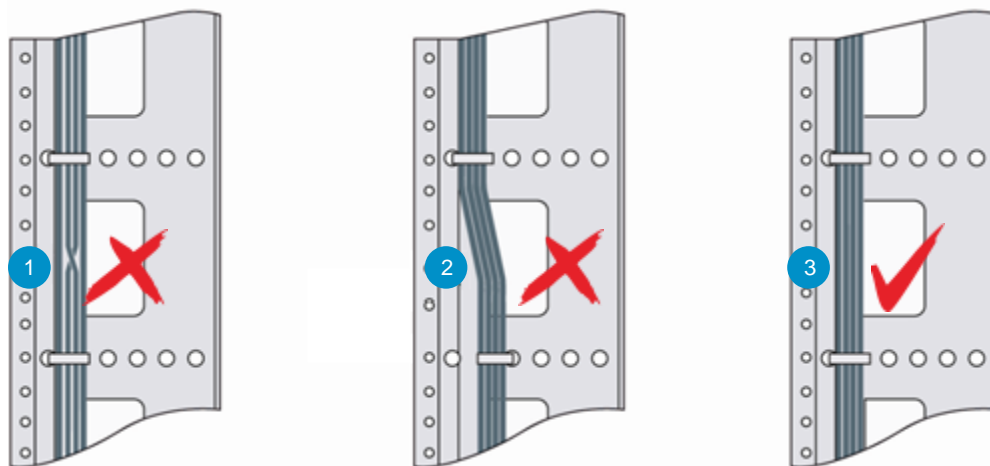
Figure 6-6 Binding Cables (1)
