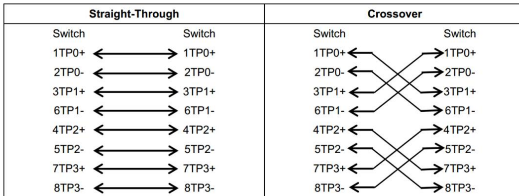
Figure 6-1 Connections of Four Twisted Pairs for the 1000BASE-T Port
