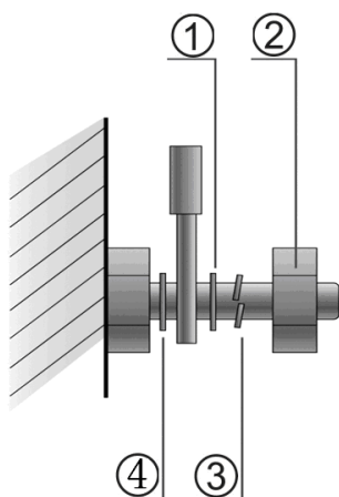
Figure 6-9 Securing Cables
