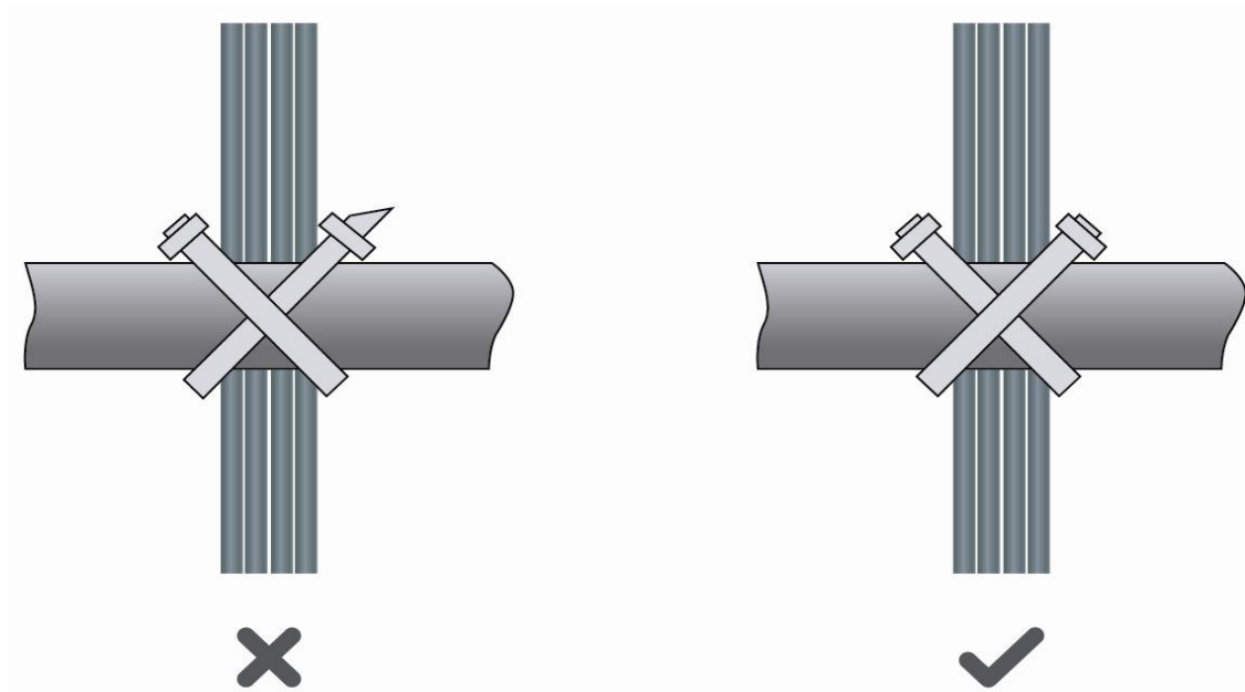
Figure 6-7 Binding Cables (2)
