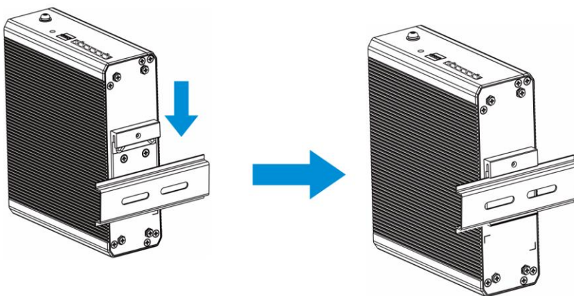
Figure 3-2 Mounting Procedure
