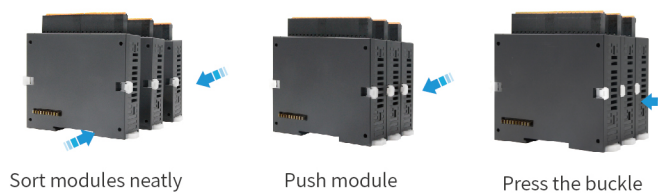
Figure 4 Snap-in buckle installation
