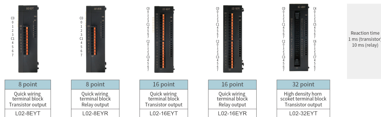
Figure 2 DIO module
