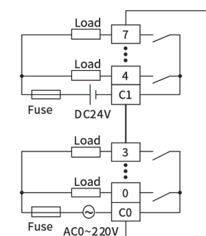
Figure 8 Relay output equivalent circuit
