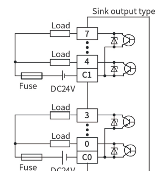
Figure 9 Transistor output equivalent circuit
