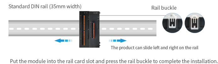
Figure 5 Rail installation
