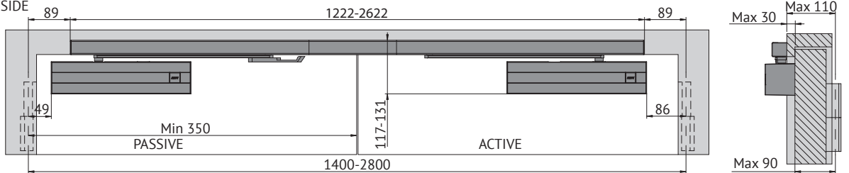
NON-HINGE SIDE WITH ANGLE MOUNTING PLATE
