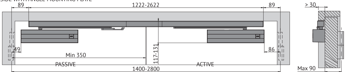
NON-HINGE SIDE WITH ANGLE MOUNTING PLATE
