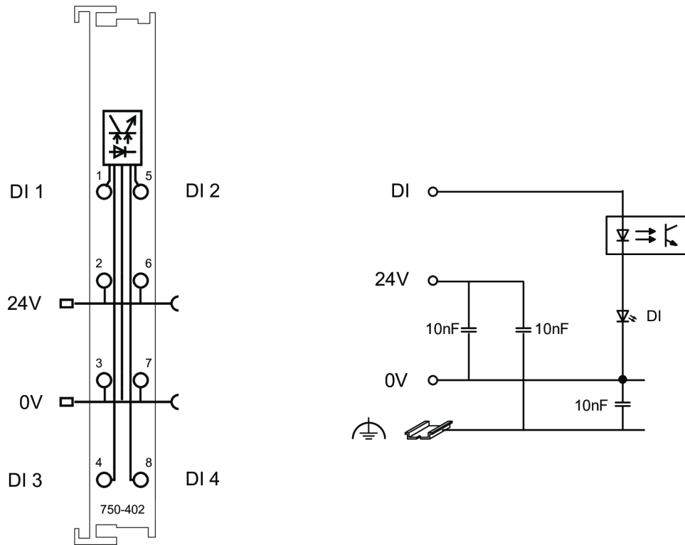
Figure 5: Circuit Diagram
