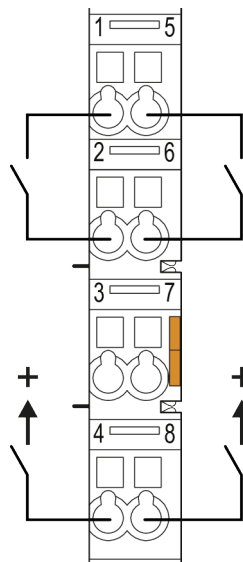
Figure 6: Example: 2-Wire Connection
