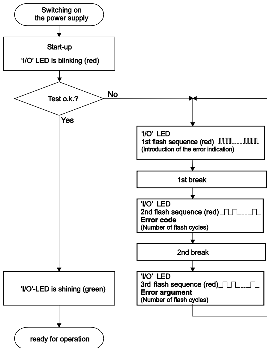
Figure 41: Node Status – I/O LED Signaling
