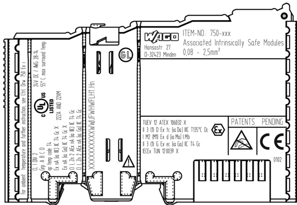
Figure 45: Marking Example for Approved I/O Module Ex i According to ATEX and IECEx
