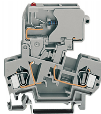
Figure 14: Fuse Modules with Pivotal Fuse Carrier, Series 281
