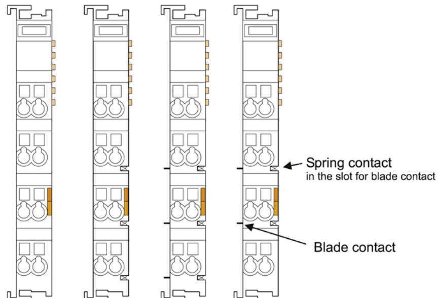
Figure 34: Example for the Arrangement of Power Contacts
