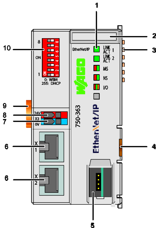
Figure 22: View FC EtherNet/IP; G4; 2ETH
