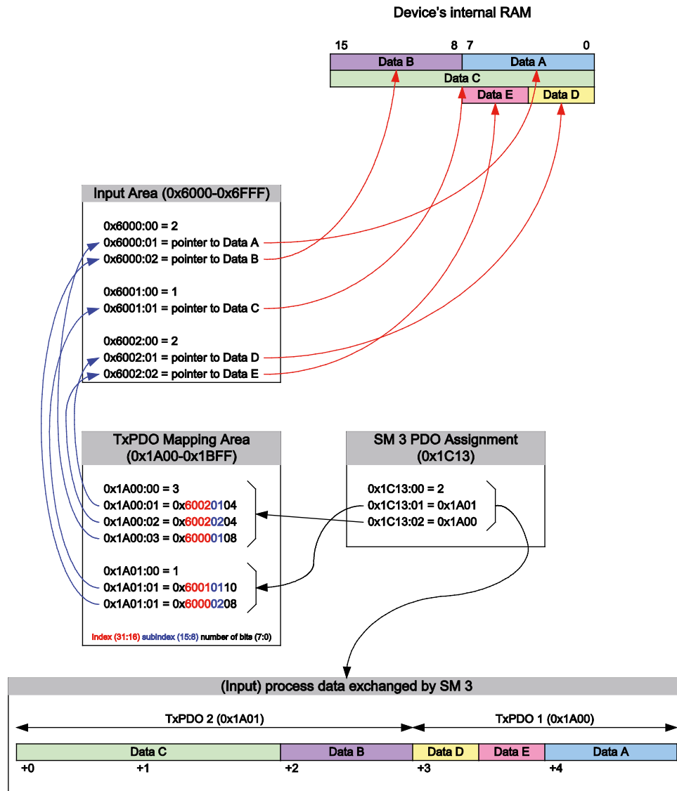
Figure 37: Example of the Principle Mapping of Process Data Using EtherCAT®
