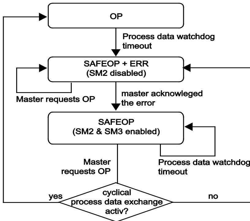
Figure 46: Error Behavior of the Process Data Watchdog
