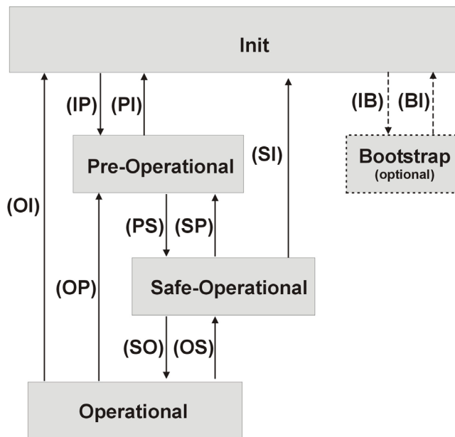
Figure 47: Status Diagram of an EtherCAT® Slave
