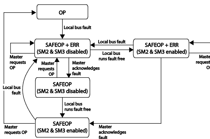
Figure 45: Behavior During a Local Bus Error
