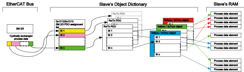
Figure 36: Mapping the Process Data
