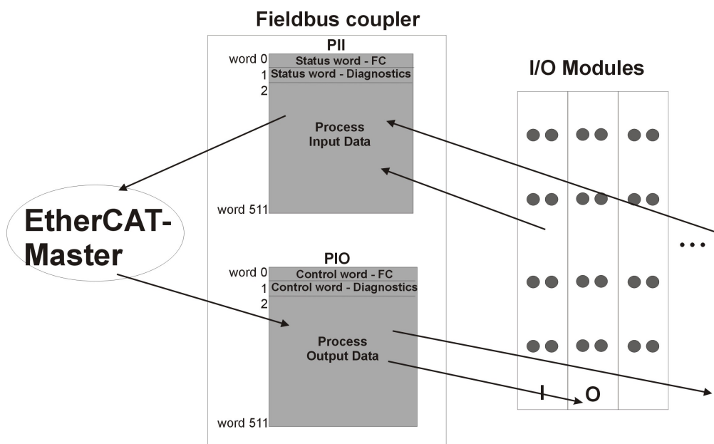
Figure 41: Memory Areas and Data Exchange of the Fieldbus Coupler
