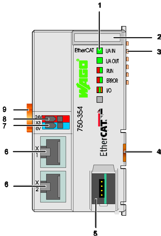
Figure 22: View EtherCAT® Fieldbus Coupler
