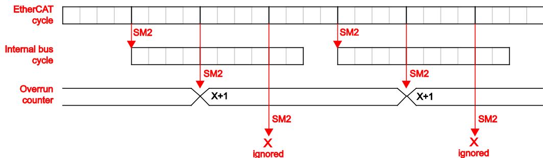
Figure 40: Overrun Counter in Subindex 11
