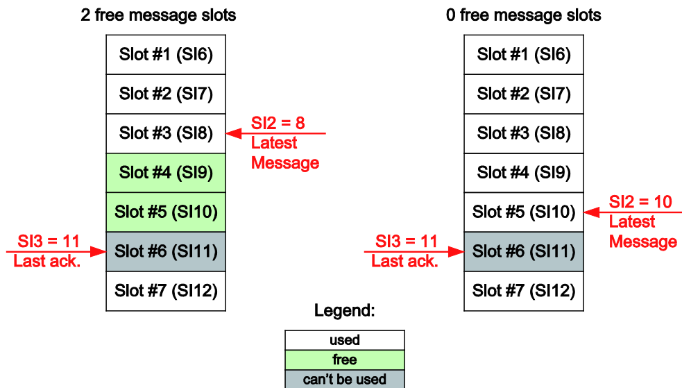
Figure 38: Number of Free Slots
