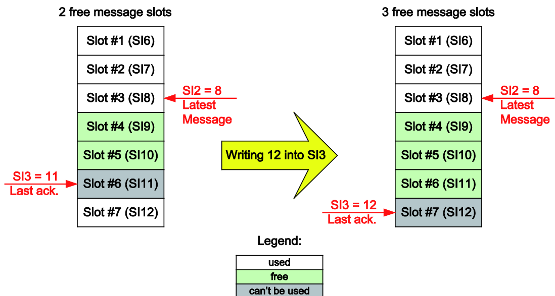
Figure 39: Acknowledgement of a Diagnostic Message
