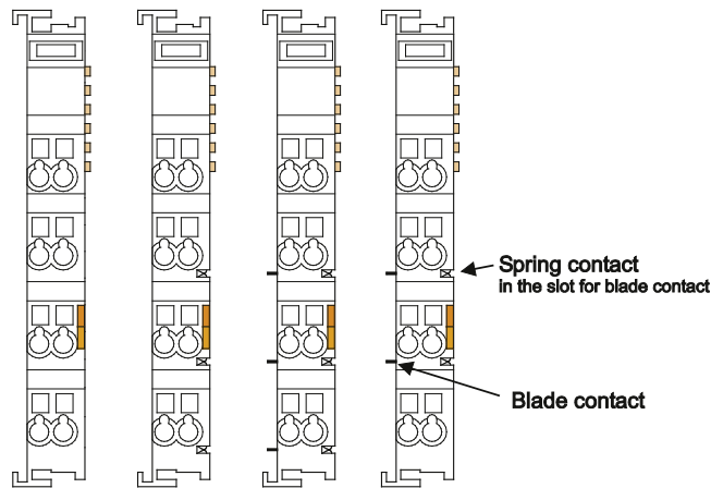
Figure 33: Example for the Arrangement of Power Contacts
