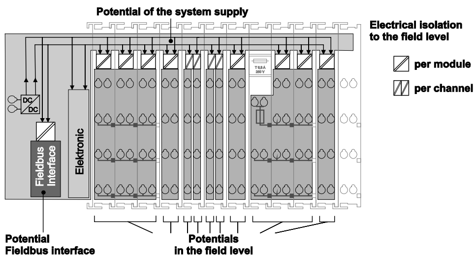
Figure 5: Isolation (Example)
