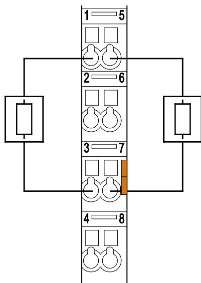
Figure 10: Connecting Diagram
