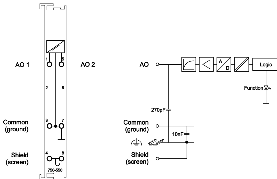
Figure 5: Schematic Diagram
