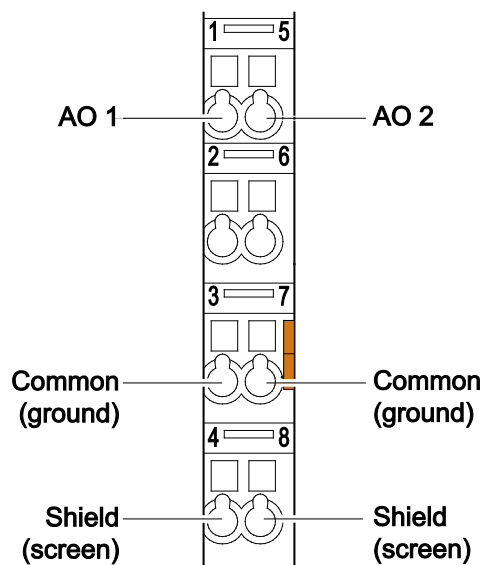
Figure 3: CAGE CLAMP® Connectors
