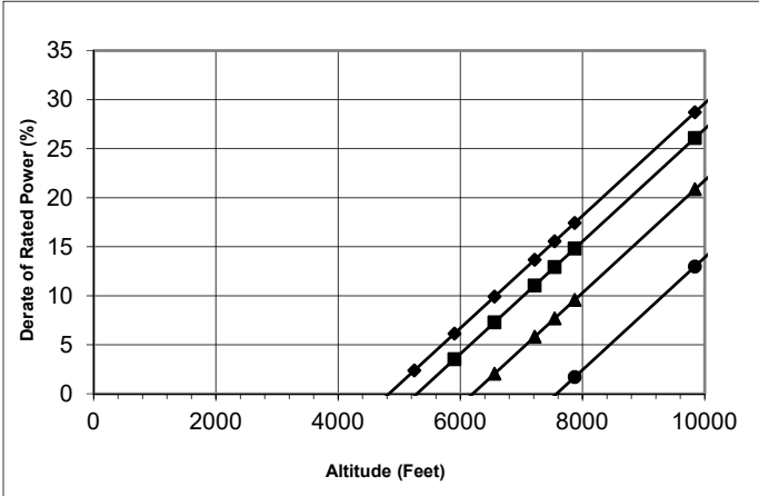
Prime Power
