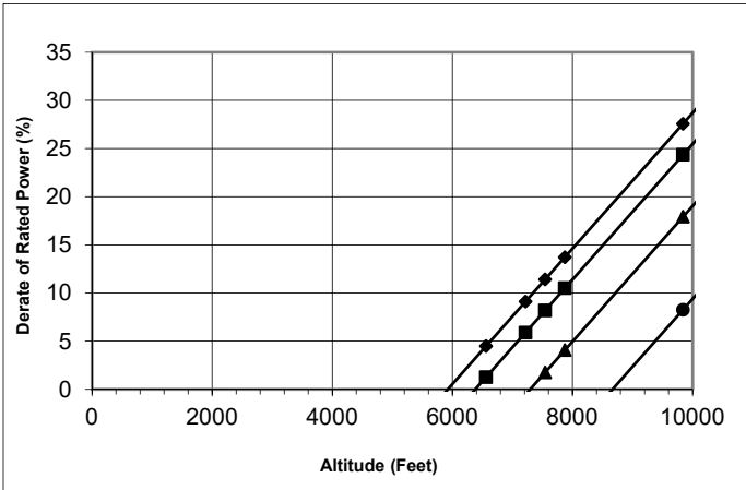
Continuous Power
