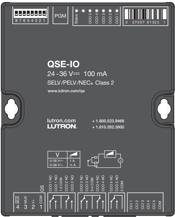
QSE-IO Contact Closure Interface
